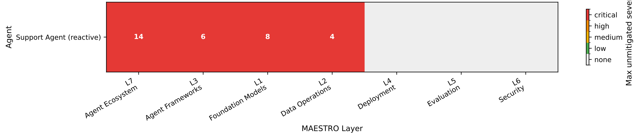
Single-Agent RAG Assistant -- Threats by Agent x Layer
